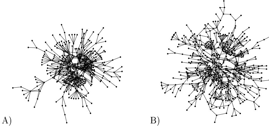
Fig. 3. A) An example of a small proteome interaction map (giant component, \Omega_\infty ) generated by the model with N = 10^3 , \delta = 0.58 , and \beta = 0.16 . B) Real yeast proteome map obtained from the MIPS database [23]. We can observe the close similitude between the real map and the output of the model.
