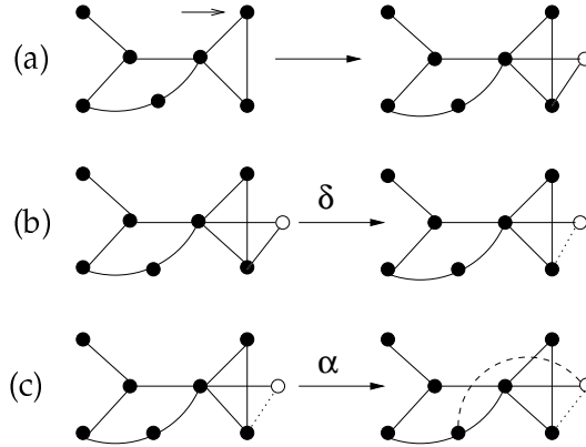
Fig. 2. Growing network by duplication of nodes. First (a) duplication occurs after randomly selecting a node (arrow). The links from the newly created node (white) now can experience deletion (b) and new links can be created (c); these events occur with probabilities \delta and \alpha , respectively.
