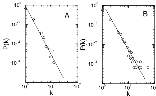
Fig. 1. Degree distributions for two different data sets from the Yeast proteome: A: Ref. [36]; B: Ref. [16]. Both distributions display scaling behavior in their degree distribution P(k) , i.e. P(k) \sim k^{-\gamma} , a sharp cut-off for large k and very small average connectivities: \bar{K}_A = 1.83 (total graph) and \bar{K}_B = 2.3 (giant component), respectively. The slopes are \gamma_A \approx 2.5 \pm 0.15 and \gamma_B \approx 2.4 \pm 0.21 .
