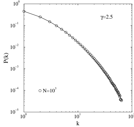
Fig. 4. Degree distribution P(k) for the model, averaged over 10^4 networks of size N = 10^3 . The distribution shows a characteristic power law behavior, with exponent \gamma = 2.5 \pm 0.1 and an exponential cut-off k_c \simeq 28 .
