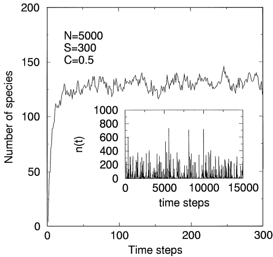
Fig. 1. An example of the time evolution of a single species (inset) from a population of N=5000 individuals and S=300 species in the pool. Here C=0.5 and \mu=5 \times 10^{-3} . We can see a wide spectrum of fluctuations in n(t) . Main figure: the number of species present in the simulated ecosystem increases up to an average value \langle S \rangle \approx 125 imposed by the matrix connectivity.
