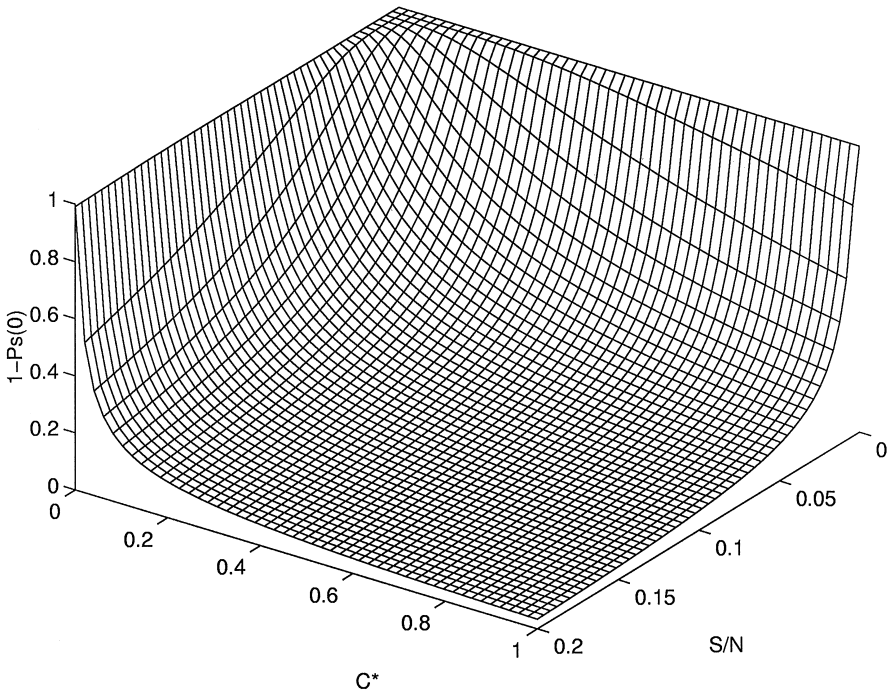
Fig. 3. Fraction of remaining species at steady state as a function of S/N and connectivity ( N = 50,000 , \mu = 0.001 ). In this parameter range, hyperbolic-like behavior can be observed for high values of S/N .
