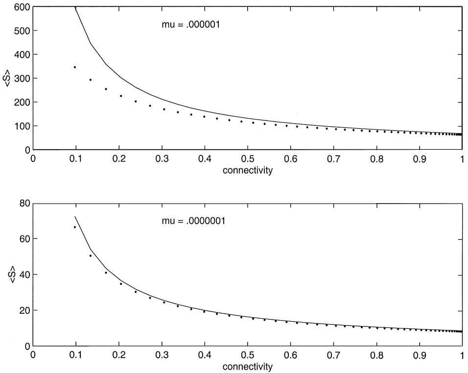
Fig. 4. Scaling between number of species and connectivity: here two different plots are shown, for N = 5 \times 10^6 , S = 500 and for different values of \mu . Dots and solid lines indicate the exact solution ( \langle S \rangle = (1 - P(0))S ) and the approximation (11), respectively.
