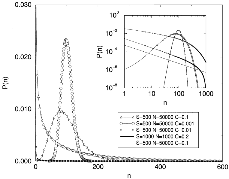
Fig. 2. Stationary probability distribution P_s(n) obtained from (4)–(6), with \mu = 10^{-3} . For different values of S/N and C we get different stationary distributions. For S = 500, N = 50,000 and different connectivities, we get Gaussian ( C = 0.001 ), log-normal ( C = 0.01 ) or power laws ( C = 0.1 , here with a strong bending). As the connectivity or S/N increases, power laws are obtained (black circles).
